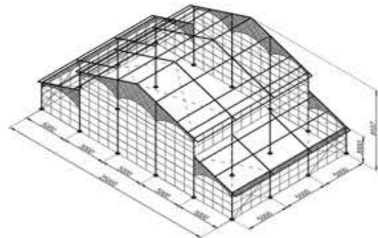
Atrium Tent Frame
